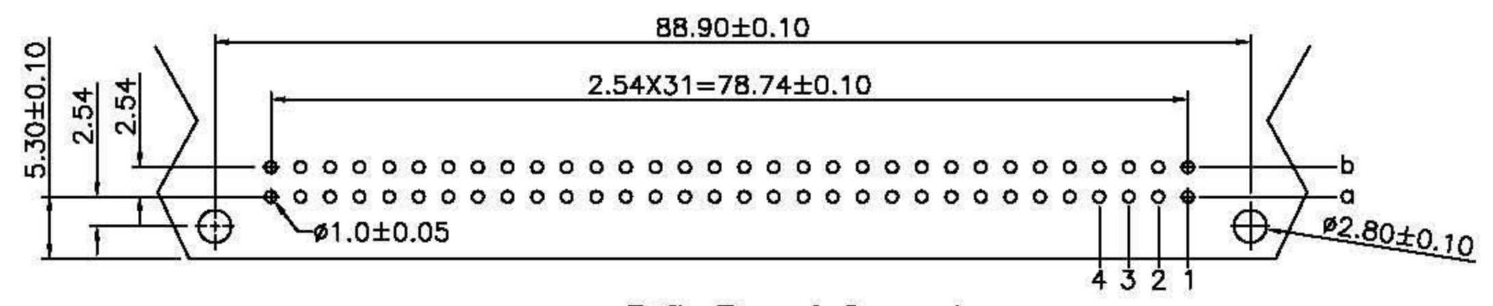
P.C. Board Layout
